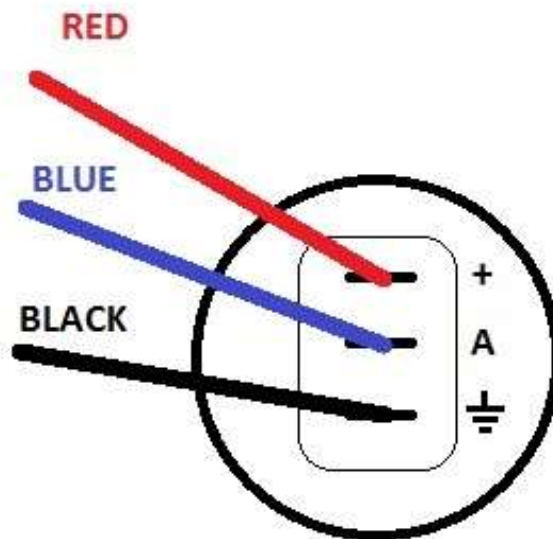
Scheme of connection.
